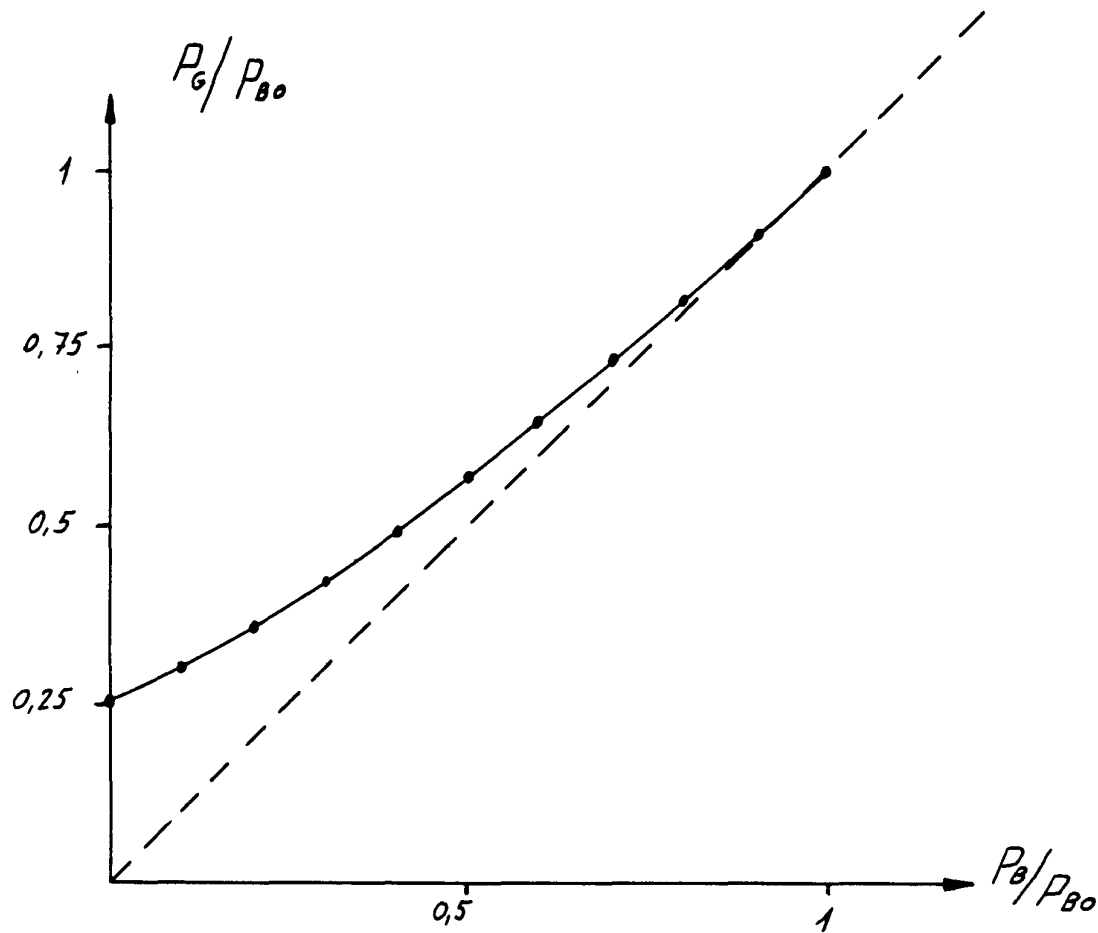
Fig. 2 Generator power for P_B < P_{B0}
