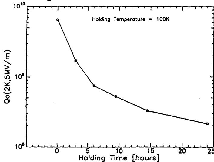
Figure 6 Q degradation due to hydrogen contamination : time dependence of degradation at 100 K (from ref. 43).
