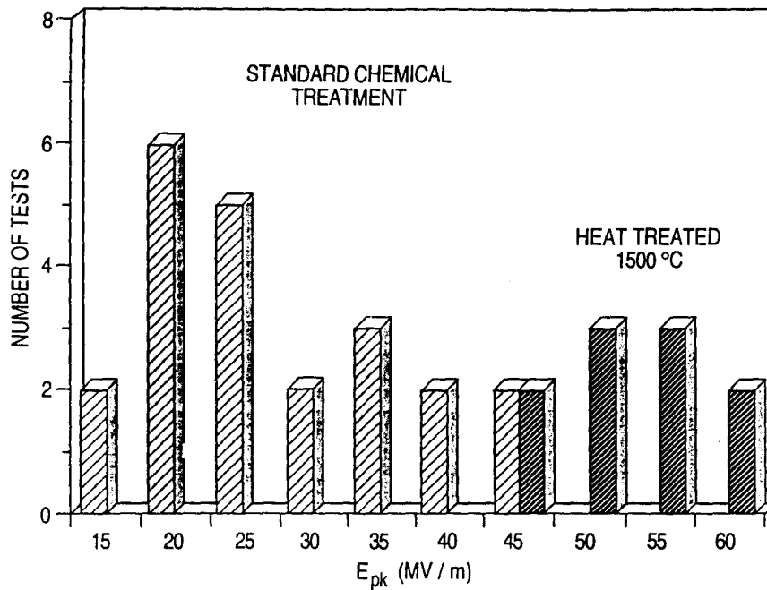
Figure 4 Benefits of the heat treatment on single cell niobium cavities at Cornell (from ref. 1).
