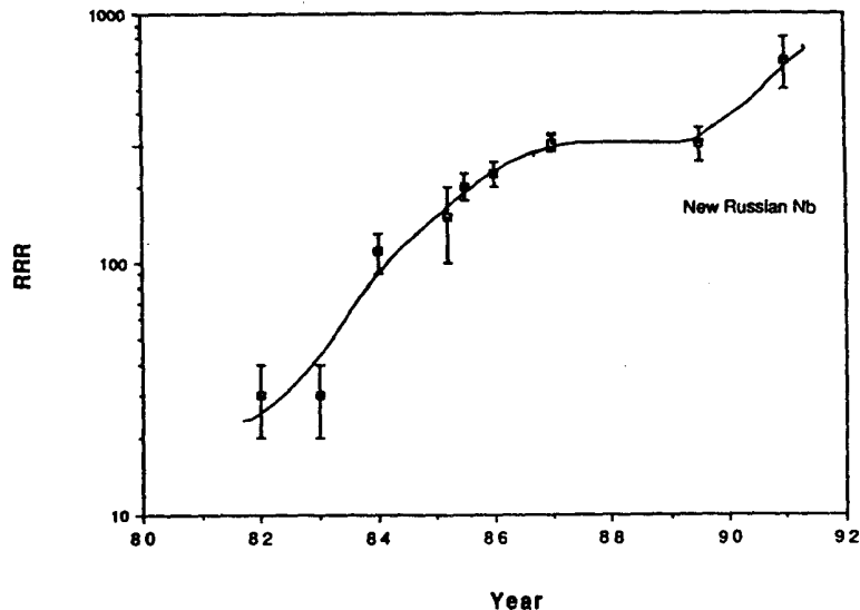
Figure 5 Progress on the purity of commercially available niobium (from H. Padamsee, private communication)
