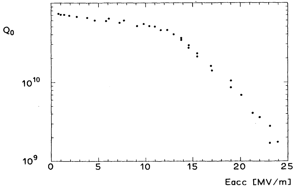
Figure 7 Very high Q-value obtained in a 3 GHz single-cell niobium cavity at Wuppertal (from ref. 44).
