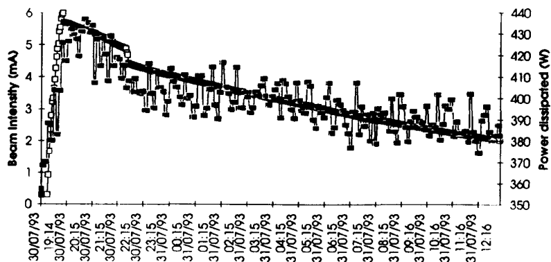
Fig 6 :Beam induced heat load.
