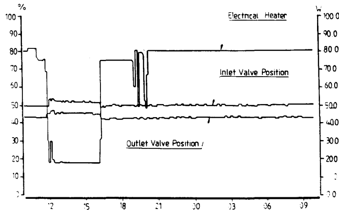
Fig. 3 : RF heat load compensation before Q value tuning versus time (hours)
