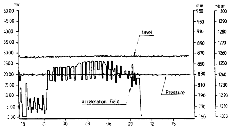
Fig. 2 : Stability of the Helium bath in a module
