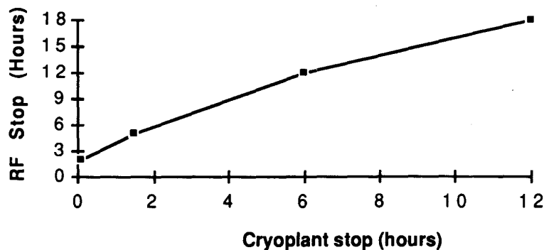
Fig 7 : Observed relation between duration of cryoplant stops and interruption of RF services
