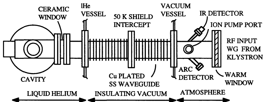
FIGURE 4: CEBAF waveguide transitions (not to scale).
