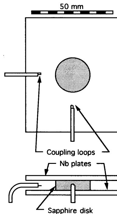
Figure 1. Schematic of the dielectric resonator. The coupling loops can be adjusted before testing. The clamp and carbon resistors have been omitted for clarity. The resonator is completely immersed in liquid helium during testing.
