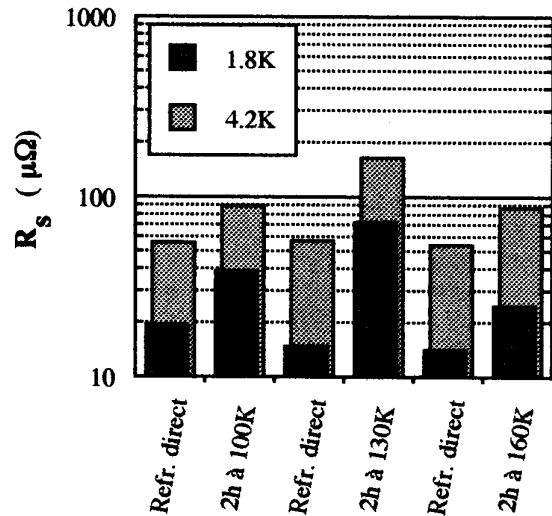
Figure 6. Effect of intermediate holding temperature on R s for RRR = 190, electropolished plates. The thermal cycle shown in Figure 5 was used for each pair of measurements. Measurements were made at 9.52 GHz.
