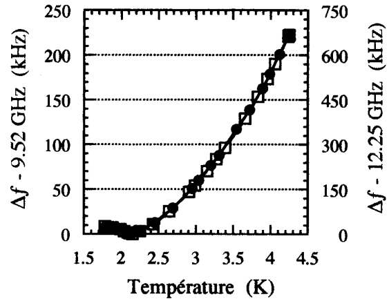
Figure 2. Temperature dependence of the resonance frequencies. The filled symbols correspond to the 9.52 GHz mode. The frequency differences for each mode are calculated relative to the frequency at 2.2K.
