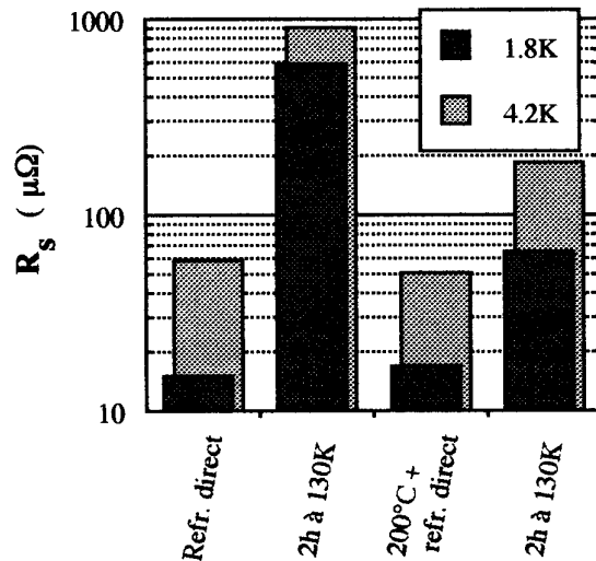
Figure 9. Effect of intermediate holding temperature on R_s for RRR = 190, chemically polished plates. The plates used to generate the data in Figure 7 were vacuum heat treated at 200°C for ~2 hours. Measurements were made at 9.52 GHz.
