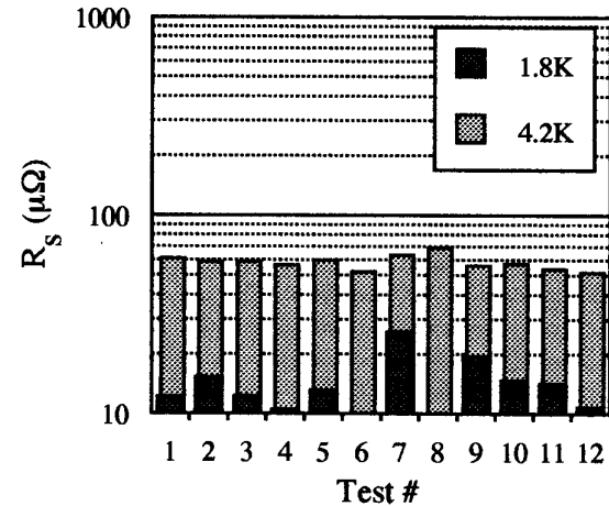
Figure 3. The results of twelve different measurements of surface resistance. The resonator was cooled quickly from room temperature for each test. All measurements were made at 9.52 GHz. Tests 1-5 used chemically polished, high RRR plates. Tests 6-8 used chemically polished, low RRR plates. Tests 9-12 used electropolished, high RRR plates. R_s at 1.8K was not measured in tests 6 and 8.
