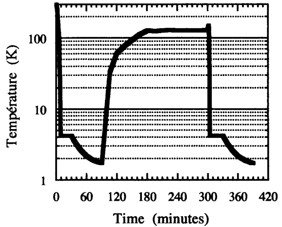
Figure 5. Typical thermal cycle of the dielectric resonator.
