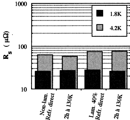
Figure 10. Effect of cold-work on R_s for RRR = 30 plates. The plates were tested at 5 mm thickness, then rolled to 3 mm thickness and tested again. The plates were chemically polished before each series of tests.
