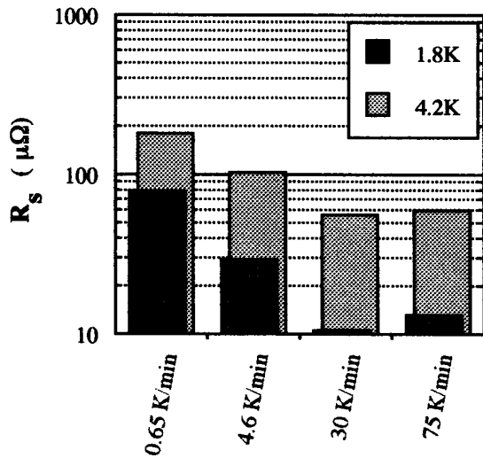
Figure 4. Effect of cooling rate on the surface resistance of RRR = 190 niobium at 9.52 GHz. The plates were cooled directly from room temperature to 4.2K.
