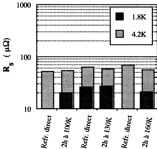
Figure 8. Effect of intermediate holding temperature on R_s for RRR = 30, chemically polished plates. The thermal cycle shown in Figure 5 was used for each pair of measurements. R_s at 1.8 was not measured for the first and fifth tests shown. Measurements were made at 9.52 GHz.
