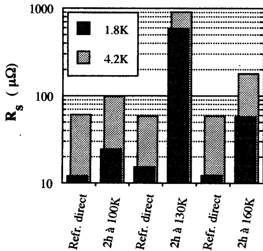
Figure 7. Effect of intermediate holding temperature on R_s for RRR = 190, chemically polished plates. The thermal cycle shown in Figure 5 was used for each pair of measurements. Measurements were made at 9.52 GHz.
