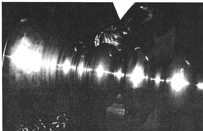
Fig. 5 Forming a multicell Al cavity by spinning [12]
