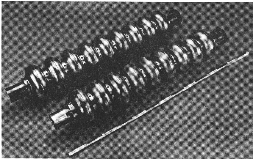
Fig. 1 9-cell cavity for TTF as example of Nb cavity production
