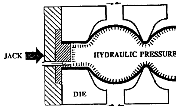
Fig. 6 Principle of hydroforming a cavity from a tube: the hydraulic inner pressure extends the tube diameter, the axial force supports the flow of material from small to large diameter.
