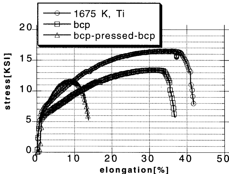
Fig. 2 Tensile measurement of Nb after different treatments [4]
