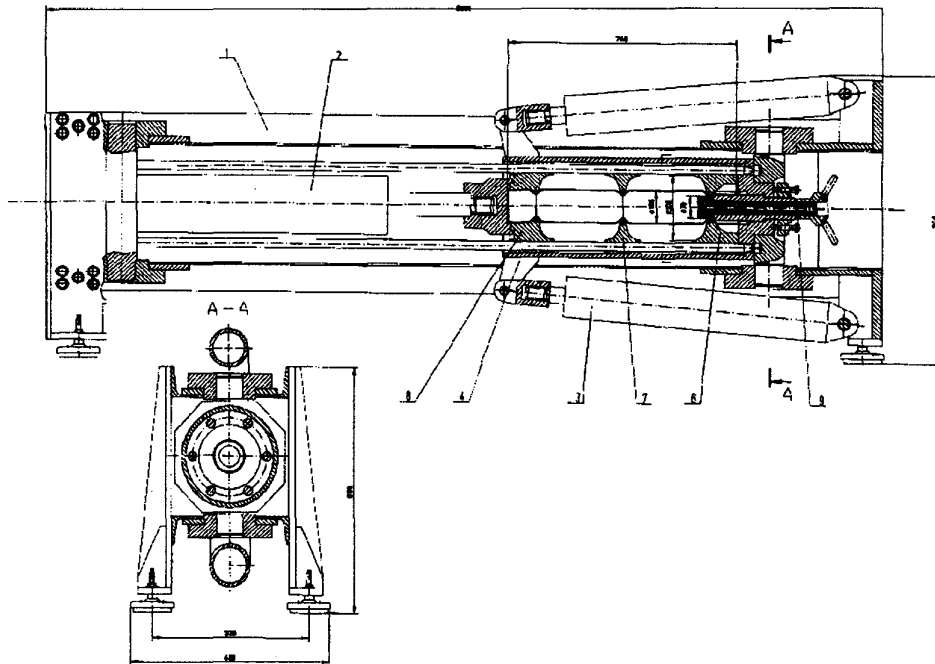
Fig. 7 Layout of a tool to hydroform multicell Nb cavities (DESY/INR, Moscow)
