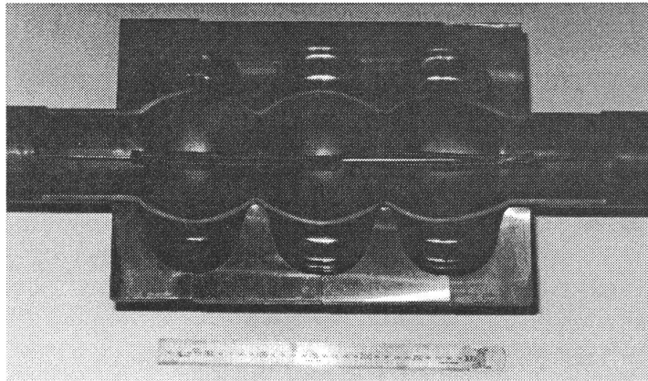
Fig. 3 Cut of a tube and a tool after first explosive forming into a 3-cell cavity [11].
