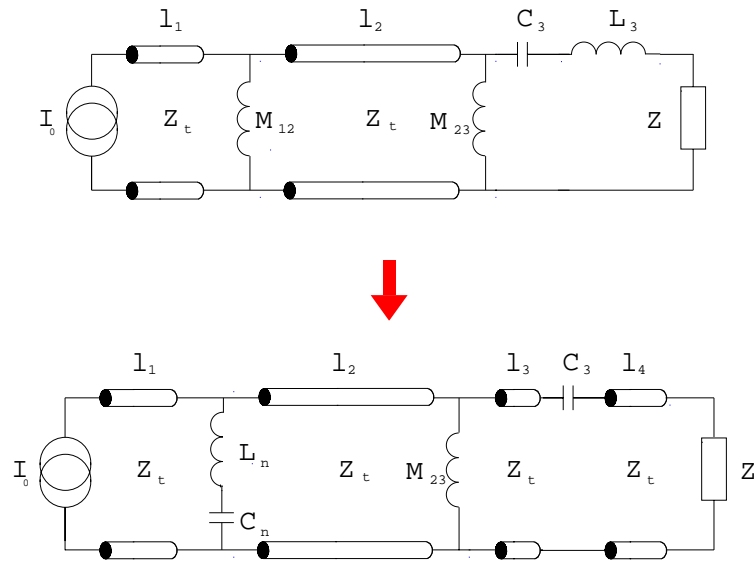
Figure 9: Equivalent circuits of the broadband coupler
