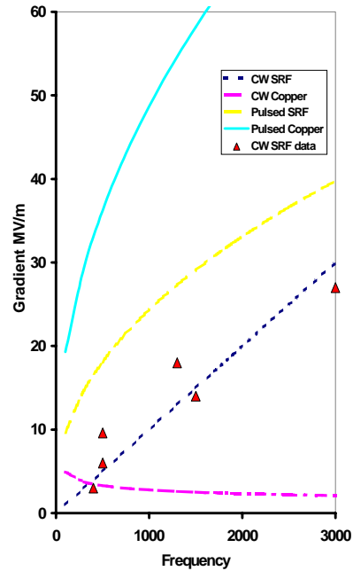
Figure 3: Gradient limits for pulsed and CW copper and srf linacs assumed in the stability calculations below.
