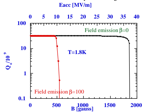
Figure 6 Q_0 versus Field plots for the Trasco cavity at 1.8 K, two different Heat generation scenarios; \beta=100 Field emitted electrons heating; \beta=0 no electrons.
