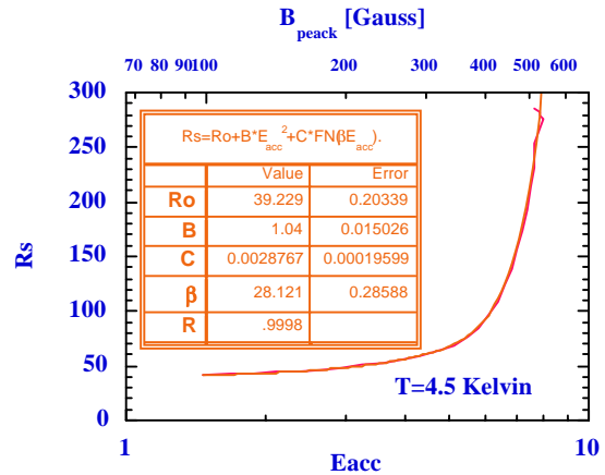
Figure 3, best fit of the losses of the cavity at 4.5K, at Low field Q(E)~Ro+B*E acc 2
