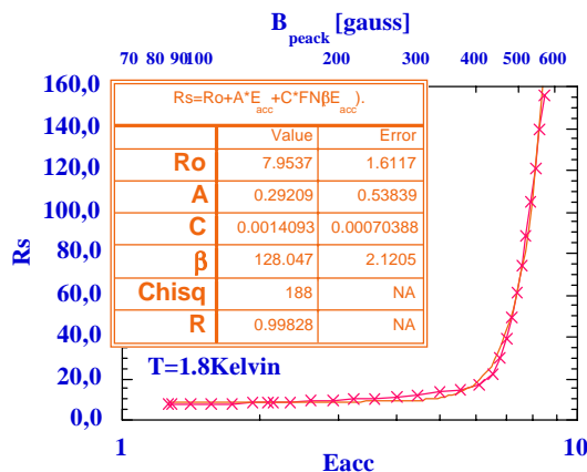
Figure 2, best fit of the losses of the cavity at 1.8K, at Low field Q(E)~Ro+A*Eacc
