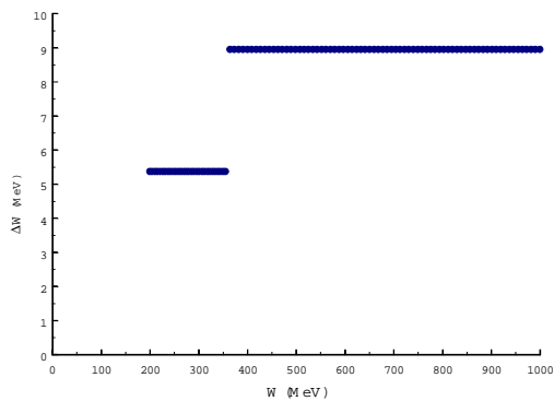
Figure 4. Energy gain per cavity versus energy.
