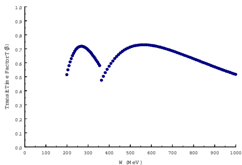
Figure 5. Cavity transit-time factor versus energy.
