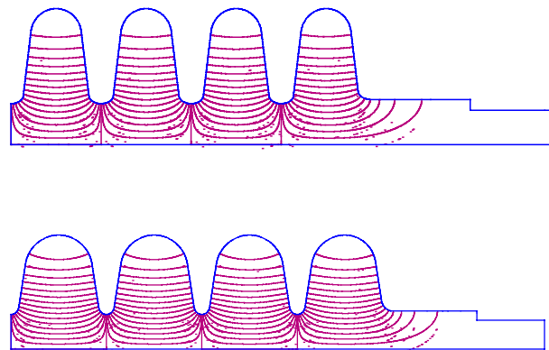
Figure 2. SUPERFISH generated cavity shapes for \beta_G = 0.61 (top) and \beta_G = 0.76 (bottom) for half of an 8-cell cavity. The contour lines correspond to constant values of the magnetic field H_\phi . The electric field is parallel to these contours.
