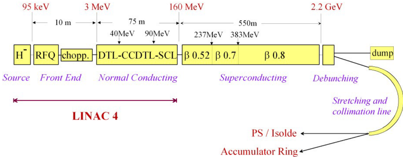
Figure 3: SPL schematic layout (original design).
