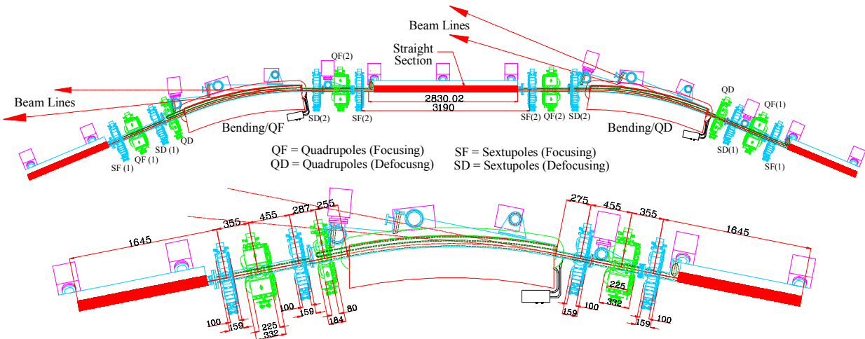
Figure 3: The arrangement of the magnets within the unit cell of SESAME IV storage ring.
