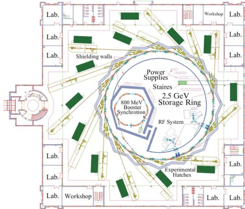
Figure 1: The layout of the ground floor of the SESAME building and the storage ring in the eccentric location, showing the beam lines from the 13 insertion device and from the bending magnets.
