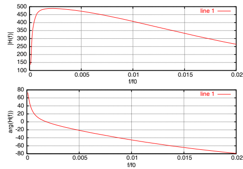
Figure 4: Characteristics of introductory IIR filter used in the longitudinal feedback
