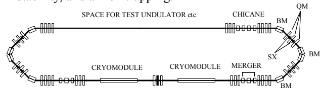
Figure 2: A prototype design of the return loop for the test ERL.
