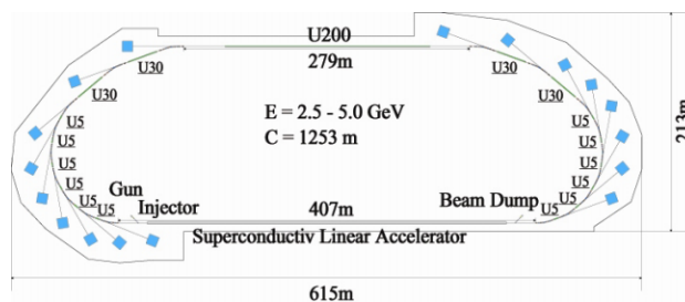
Figure 1: Conceptual layout of 5 GeV ERL.
