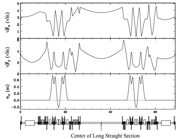
Figure 3: Typical optical functions along the return loop. Periodic condition was assumed.
