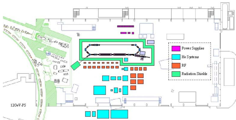
Figure 5: A temporary layout of the test ERL which is fit to the East Experimental Hall of the 12-GeV PS.
