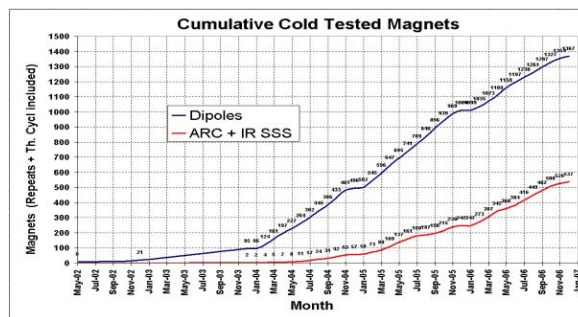
Figure 4: Cumulative Cold Tested Magnets.
