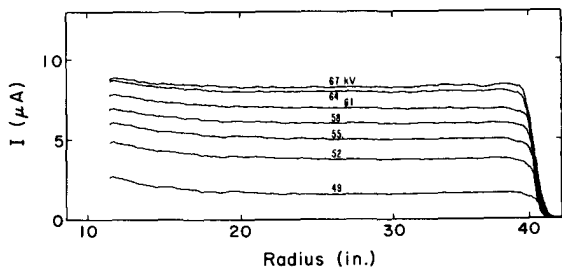
Fig. 5 The 130 MeV \alpha beam; effect of varying the dee voltage.
