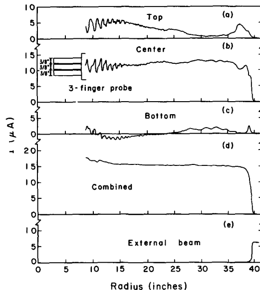
Fig. 6 The 65 MeV \alpha beam with which an extraction efficiency exceeding 40% has been obtained.
