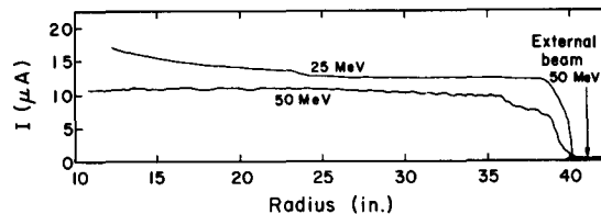
Fig. 12 The 25 and 50 MeV proton beams.
