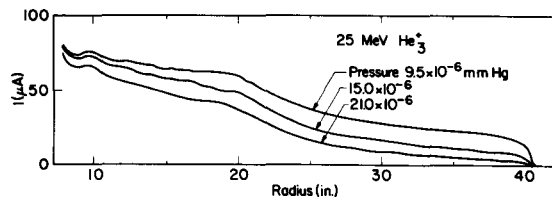
Fig. 13 Attenuation of 25 MeV \text{He}^{3+} beam.
