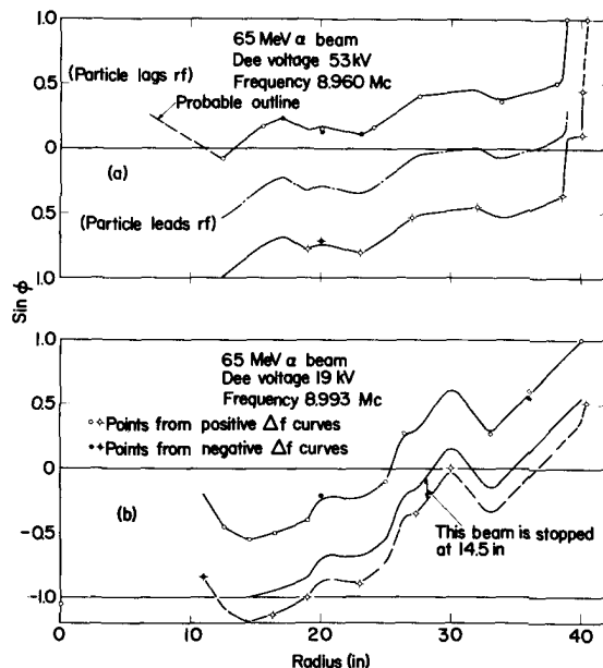
Fig. 8 Phase plots of the 65 MeV \alpha beam. (a) By using curves of Fig. 7. (b) By using curves made with a dee voltage of 19 kV.
