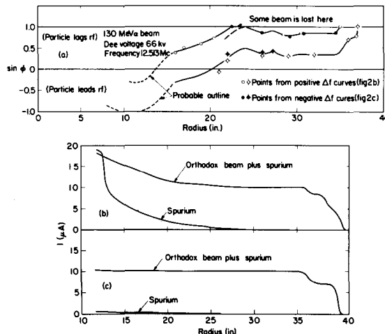
Fig. 3 Development of the 130 MeV \alpha beam. (a) The phase plot deduced from the curves of Fig. 2 (b) and (e). (b) The beam obtained after trim-coil adjustments were made. The spurious beam, obtained by blocking the orthodox beam with another probe, is also shown. (c) After center region adjustment was made to eliminate spurious.
