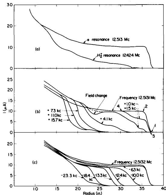
Fig. 2 Development of the 130 MeV \alpha beam. (a) The first \alpha beam obtained, with the corresponding H_2^+ beam. (b) and (c) The \alpha beam as a function of frequency.
