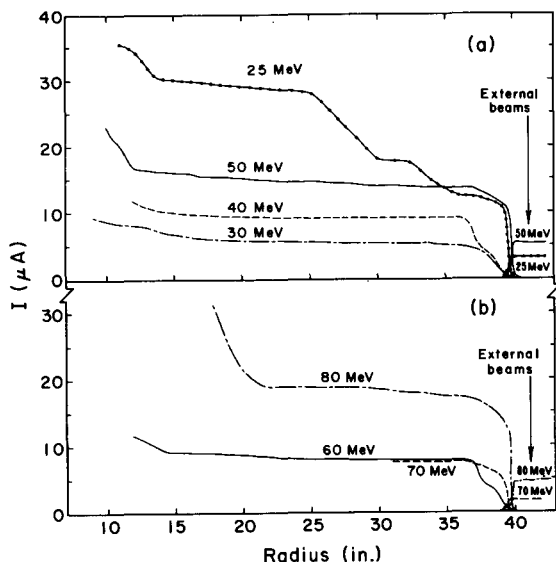
Fig. 11 The 25 to 80 MeV \alpha beam. With minor trim-coil adjustments any intermediate energy can be obtained.
