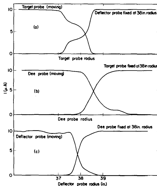
Fig. 10 Shadow measurements of the 65 MeV \alpha beam.
