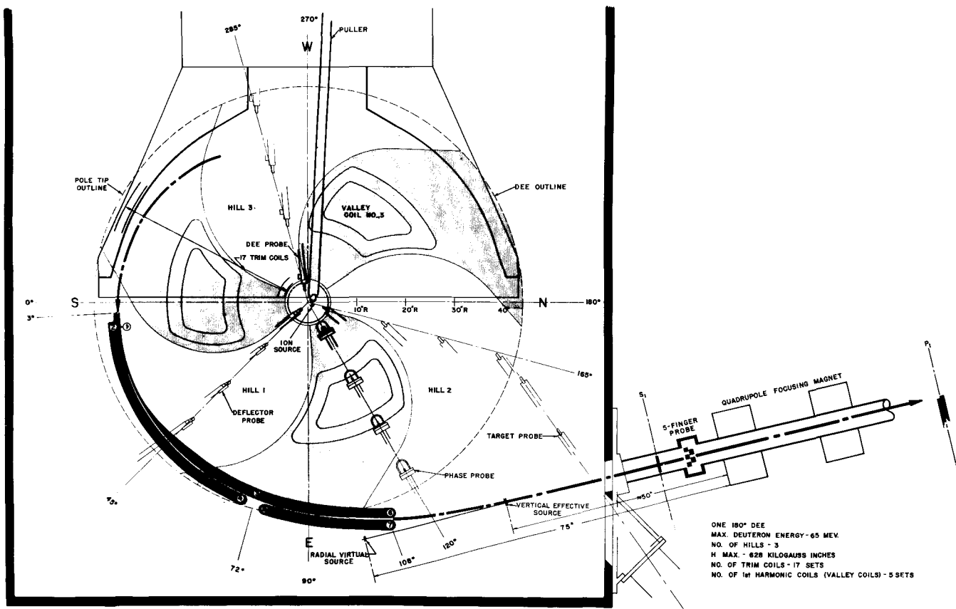
Fig. 1 Plan view of pole face.
