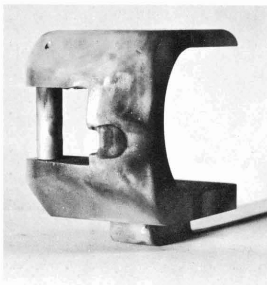
Fig. 16 Puller after 500 hours of operation.
