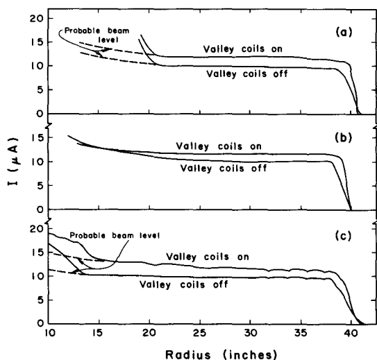
Fig. 9 Use of valley coils 1, 2 and 4 with the 65 MeV \alpha beam. Records of (a) deflector probe, (b) target probe and (c) dee probe.
