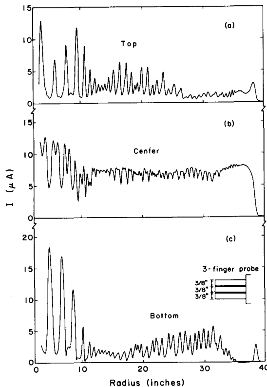
Fig. 4 Record of 130 MeV \alpha beam made with a 3-finger probe.
