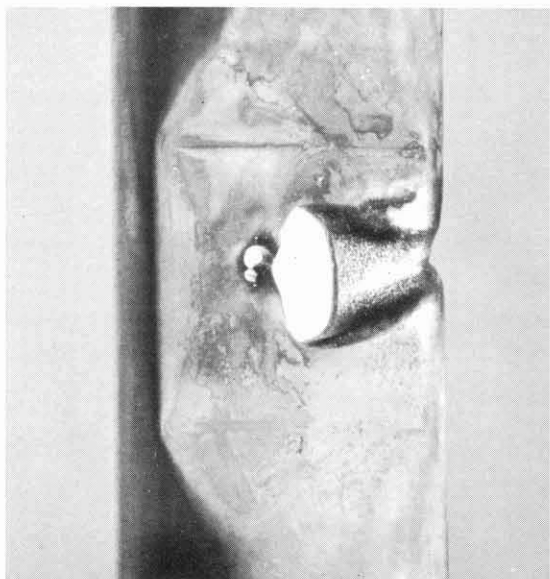
Fig. 14 Copper anode of ion source after more than 500 hours of operation.
