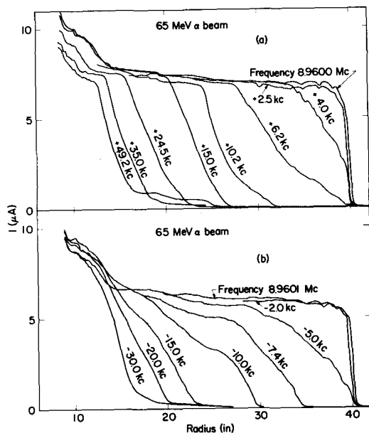
Fig. 7 The 65 MeV \alpha beam as a function of frequency.
