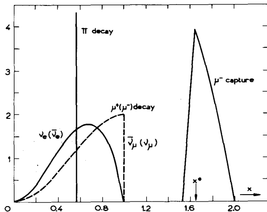
Fig. 1 Neutrino energy spectra available from 750 MeV stopped protons. The \nu_{\mu} are obtained from stopped negative muons. x = energy in units of one half the muon rest energy (U. Oberall, preprints).
