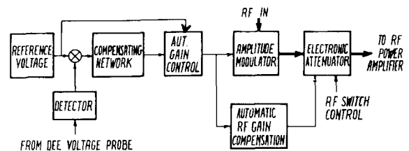
Fig. 3 : Amplitude regulation system.
