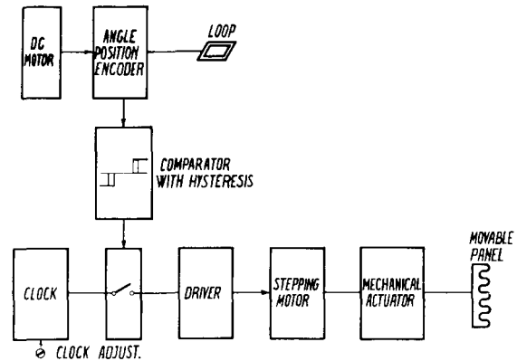
Fig. 2 : Complementary servo loop.
