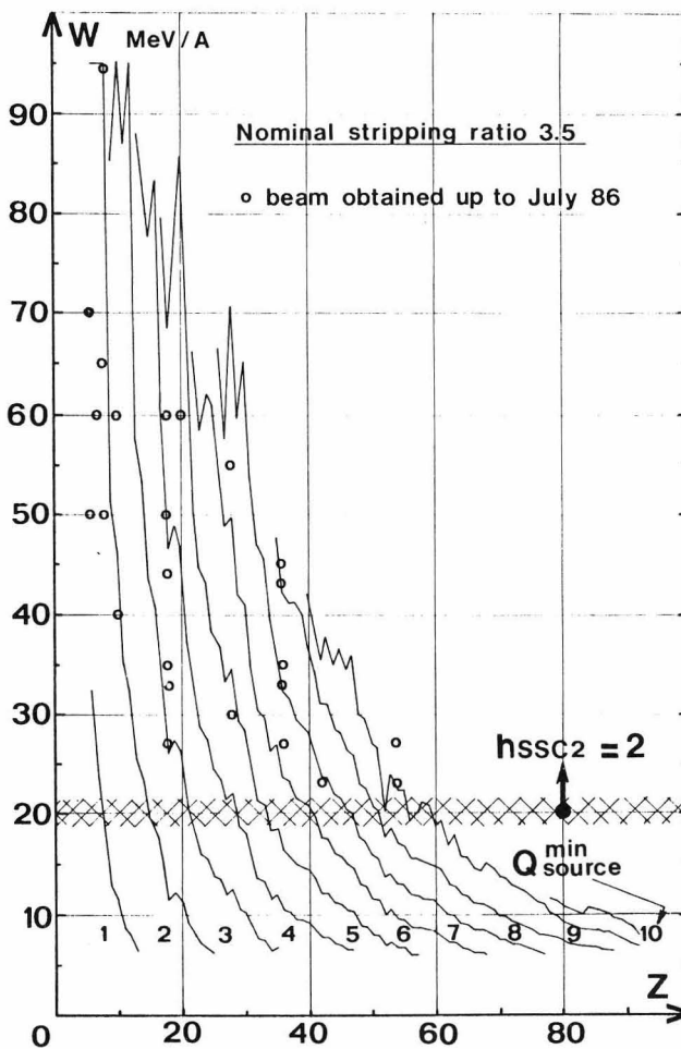
Fig.5. Energies computed (solid lines) and obtained (dots) as a function of the charge state of the PIG or ECR source. Stripping ratio 3.5.
