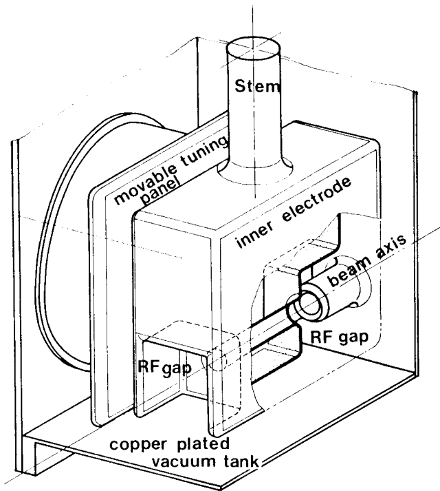
Fig.6. A view of buncher R1 with the modified RF gaps.
