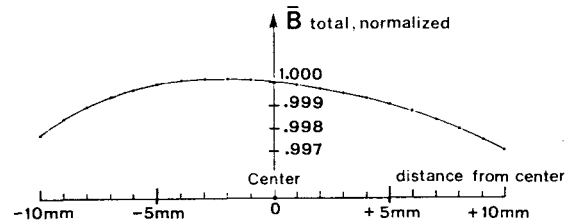
Fig.8. Magnetic septum MSi3. Top : cross-section Bottom : magnetic field averaged over the length of the septum. The curve corresponds to an average field of 2.17T on axis. The contribution of iron bars is 6.40T. Beam width is 6mm.
