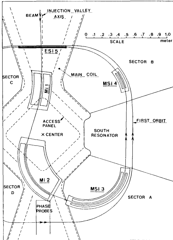
Fig.7. The new injection system will be similar to the present one. Strong fields are needed for magnet Mi2 and inductive septum MSi3.
