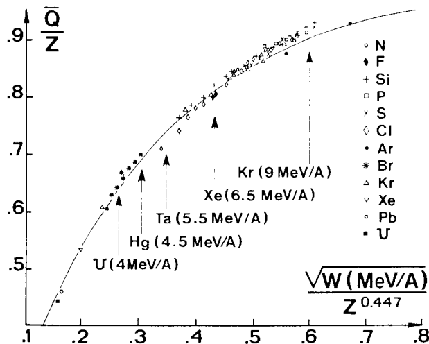
Fig.3. The solid curve is given by formula (2). Experimental data compiled by E. BARON. The arrows locate the maximum energy at the stripper for different ions in the new configuration.
