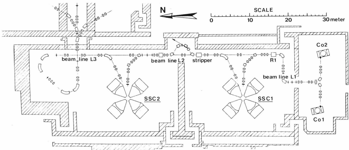
Fig.1. General lay-out of GANIL accelerator
