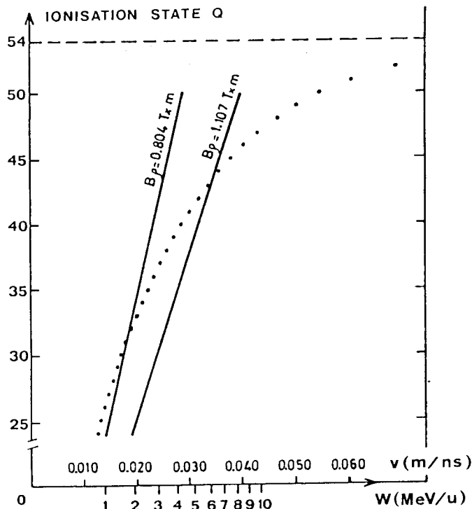
Fig.2. Most abundant charge for Xenon as a function of speed v , or energy W .
