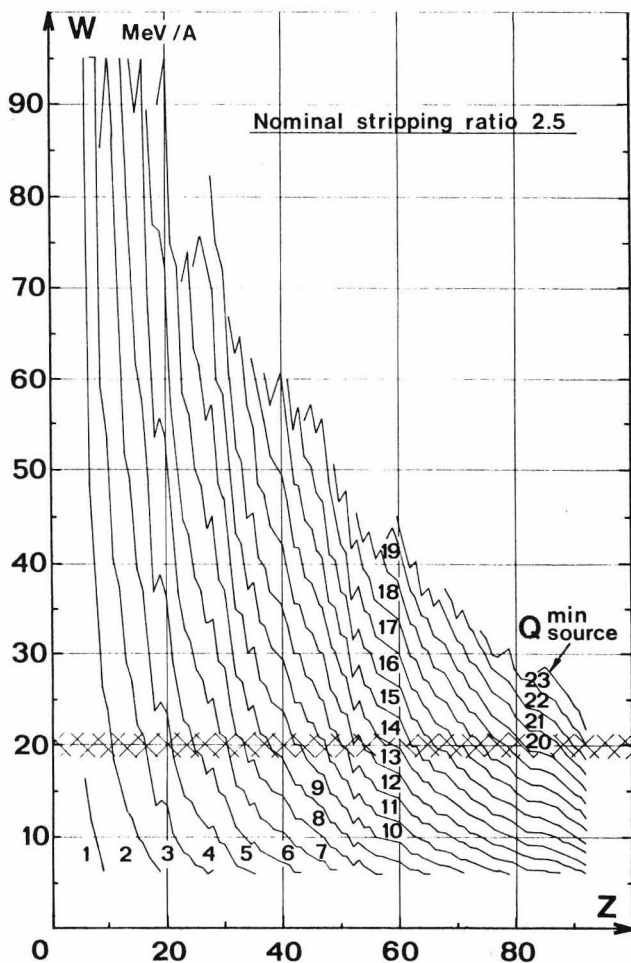
Fig.4. Energies expected at ejection of SSC2 as a function of the charge state of the PIG. Stripping ratio 2.5.
