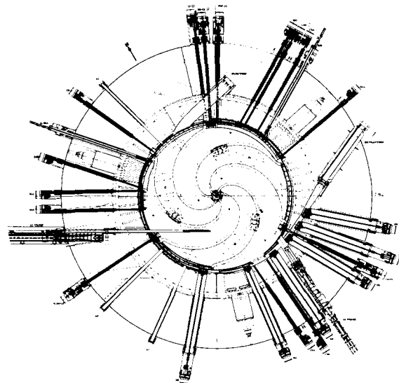
Figure 1: Mid-plane section of the K1200 showing the multiple drives associated with the extraction system elements.
