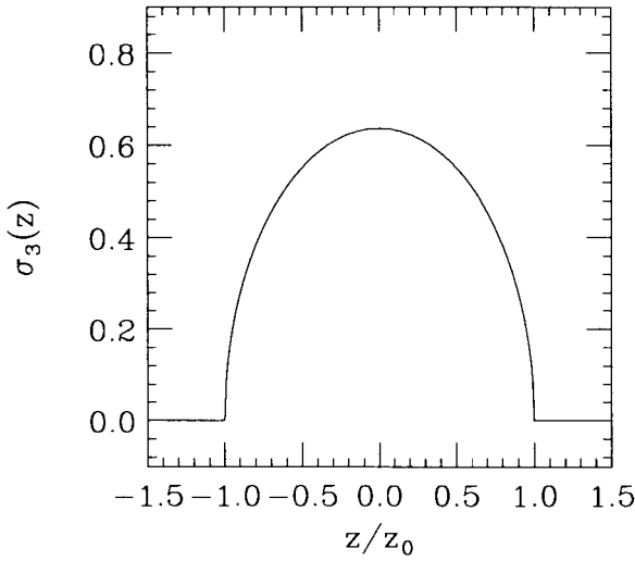
Figure 7: Charge distribution in the vertical direction used in the longitudinal space charge force calculations.
