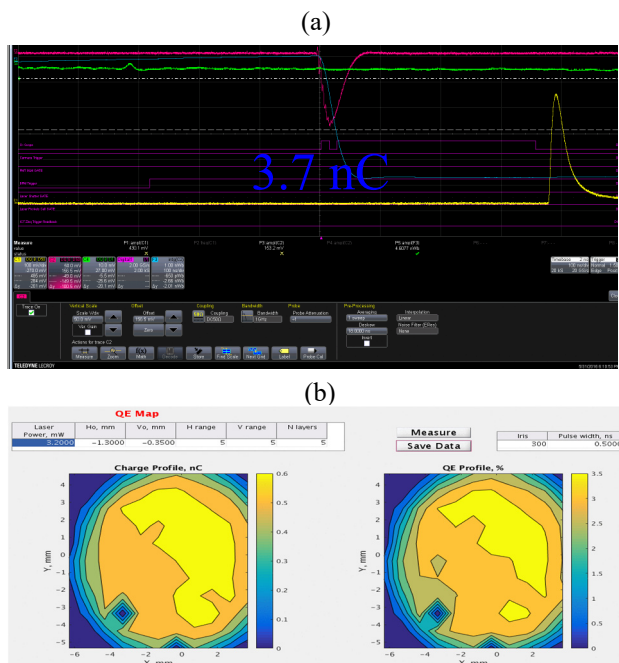
Figure 2: (a) A typical digital scope trace showing the electron bunch pulse (from integrated current transformer, red trace) and delayed trace of laser pulse (from a slow photodiode sensor); (b) a measured QE map of CsK 2 Sb photocathode after two months of operating in the SRF gun.
