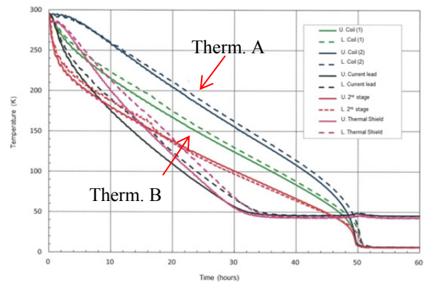
Figure 6: Initial cooling performance of the HTS magnet.
