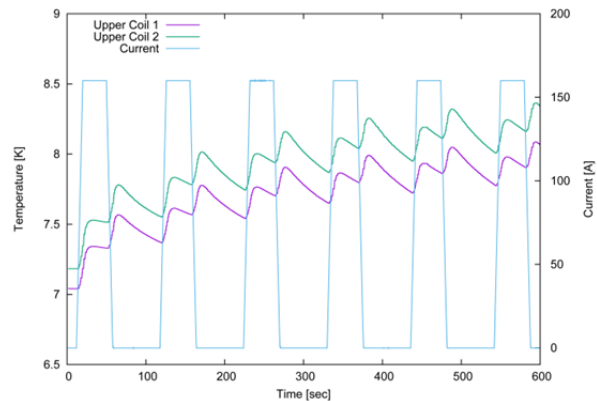
Figure 7: Temperature of upper coil during pattern operation.
