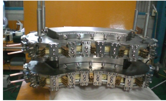
Figure 3. Photograph of the poles and coils of the model dipole magnet.
