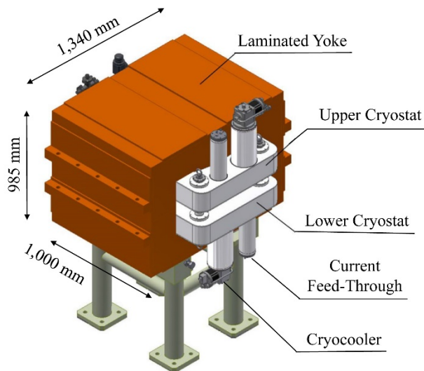
Figure 4: HTS switching dipole magnet..
