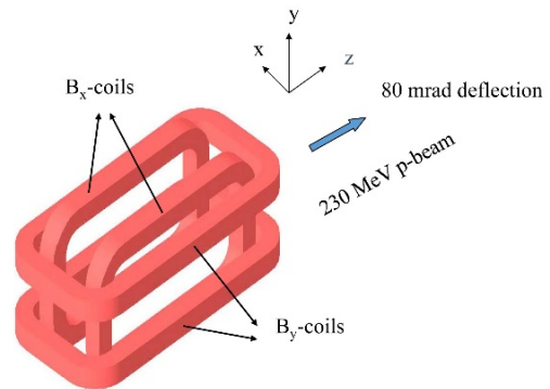
Figure 1. A schematic layout of the scanning magnet. They generate the horizontal ( B_x ) and vertical ( B_y ) field.
