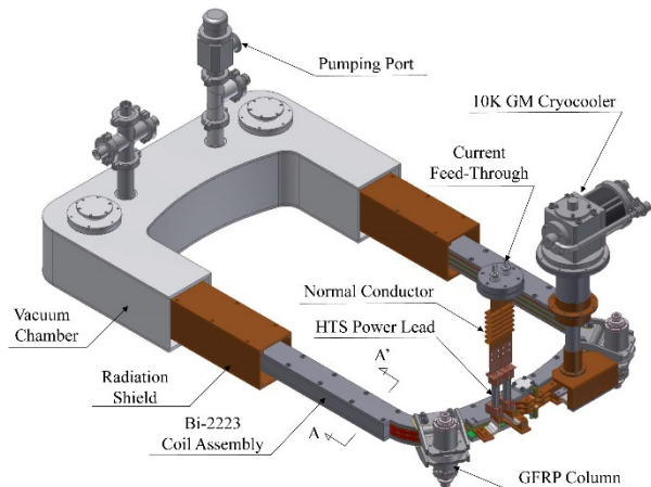
Figure 4: HTS switching dipole magnet..
