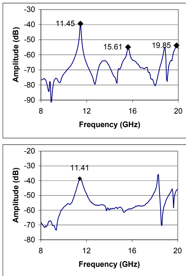
Figure 4: Frequency response of the cavity BPM.
