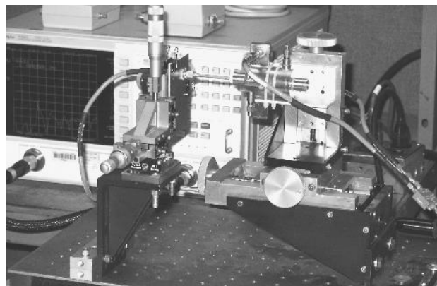
Figure 3: Cavity BPM test setup.
