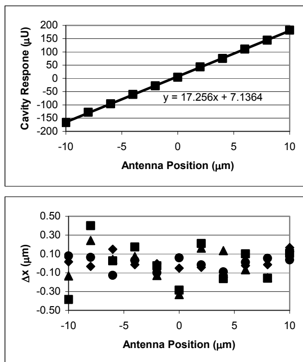
Figure 5: Top - Response of cavity BPM vs antenna position. Bottom – Difference between the calculated position and the antenna position.
