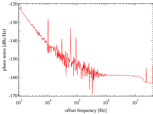
Figure 2: Measured phase noise, integrated timing jitter in a bandwidth from f_1 = 1 kHz to f_2 = 20 MHz amounts to \Delta T_{rms} = 9 fs
