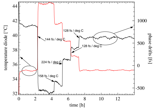
Figure 9: Phase drift dependence of photodiode
