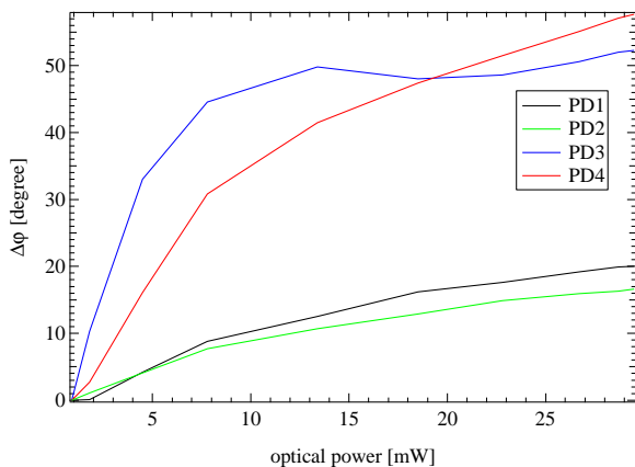
Figure 4: AM to PM characteristics of photodiodes
