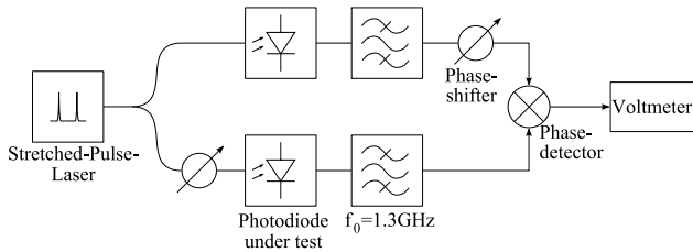
Figure 3: Setup to examine AM to PM conversion of photodiodes
