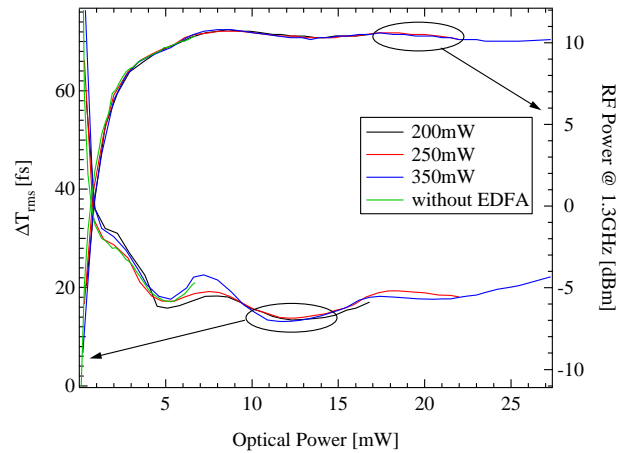
Figure 6: Integrated timing jitter and RF power of photodiode PD3 vs. optical power for different EDFA pump-powers at 980nm
