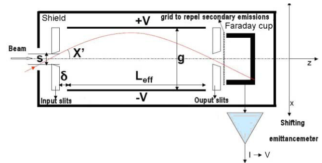
Figure 5: Schematic of the Alison emittancemeter of the L.E.B.T. and M.E.B.T.
