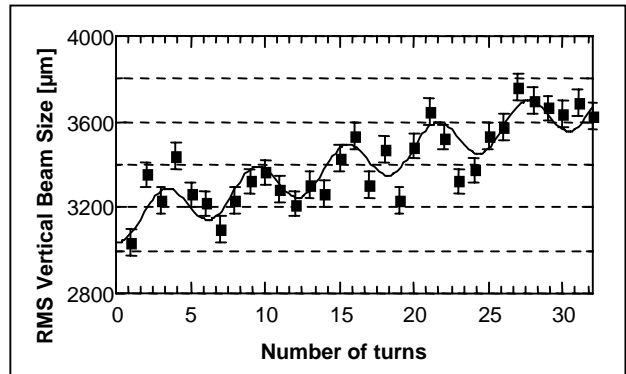
Figure 8: R.m.s. vertical beam size modulation measured over 32 turns in the SPS for a matched beam.
