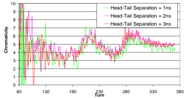
Figure 4: Turn-by-turn chromaticity for three different head-tail separations (70 GeV, hor. chromaticity = +4).
