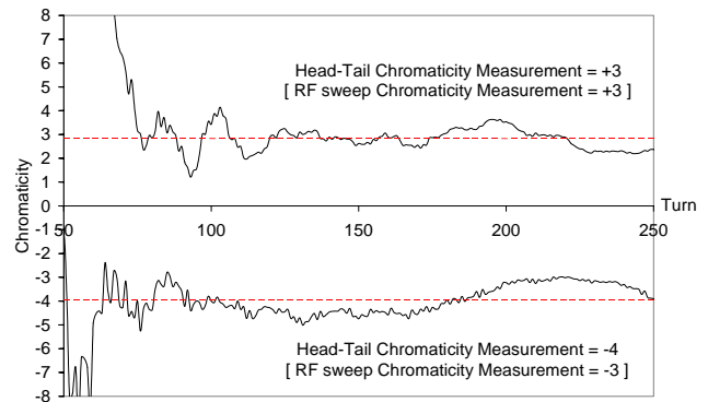
Figure 5: Turn-by-turn chromaticity for positive and negative chromaticity at 300 GeV ( \pm 1 ns head-tail separation).
