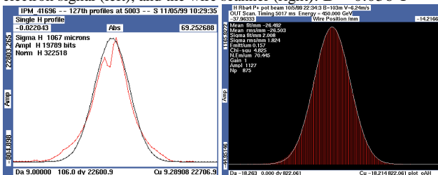
Figure 9: Corresponding profiles measured at 450 GeV.
