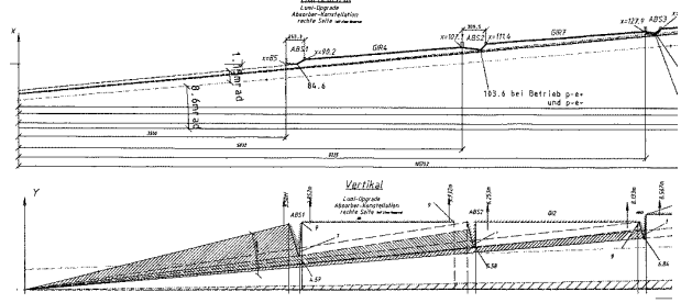
Figure 2: Locations of emergency absorbers downstream of the interaction point.
