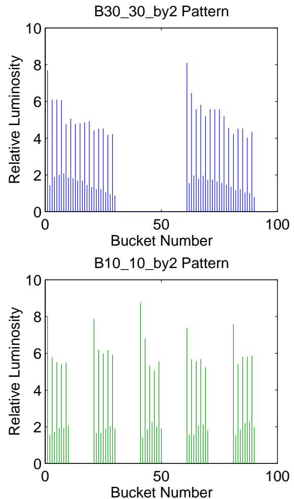
Fig. 3: Luminosity for "by 2" Pattern with Gaps. The luminosity is plotted versus the number of buckets for the first 100 buckets ("by 2"). The gaps appear to clear out the electron clouds around the positron beam, giving the next bunch more luminosity.
