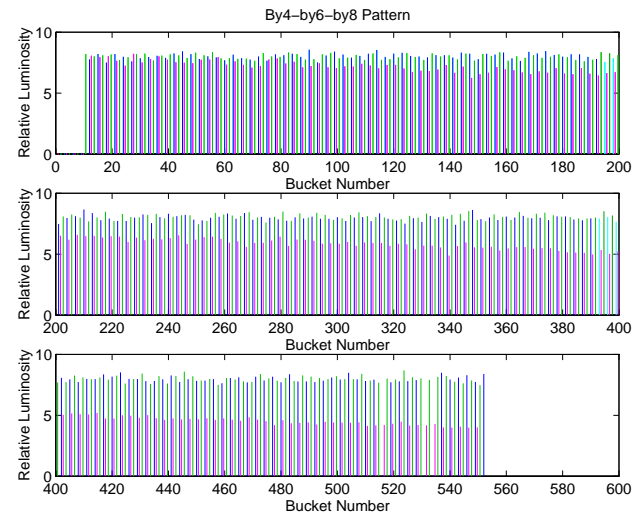
Fig. 5: The Luminosity Drop across the Fill. In most patterns there is a luminosity drop across the fill. In this 4,6,8 pattern the bunch after only 4 buckets is much less than its neighbours and with a long time constant dropping along the bunch train. Some electron bunches in the back of the train were totally kicked out after some bigger 8 bucket gaps leading to no luminosity.
