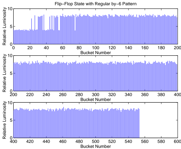
Fig. 4: Flip-Flop Behaviour in the “by 6” Pattern. The positron beam after the gap is small, blowing up the electron beam, which gives less luminosity. Later the electron cloud around the positrons blows this beam up, giving the electron beam a chance to reduce its size. This results in a higher luminosity. By adjusting the tunes it was possible to flip some bunches from one state to the other. The current distribution was flat in both rings.
