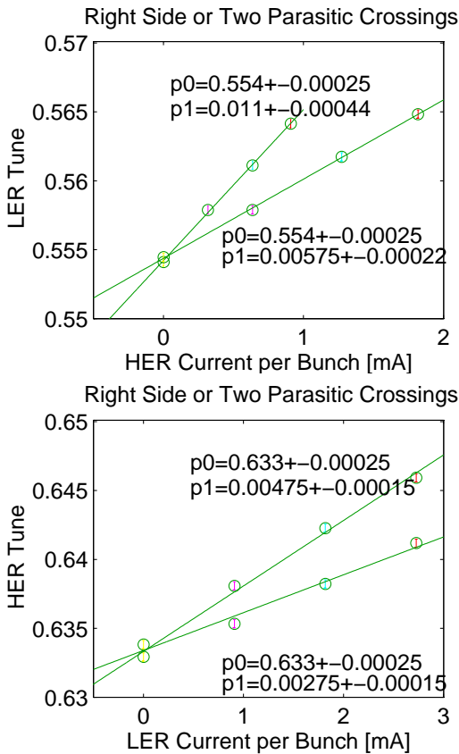
Fig. 2: Parasitic Crossing Tune Shifts. The vertical tune shifts per current ( p_1 ) for LER and HER is shown for one and two parasitic crossings.
