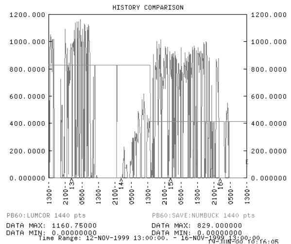
Fig. 1: Luminosity in November of 1999. The luminosity in unit of 10^{30} \text{ cm}^{-2} \text{ s}^{-1} and the number of bunches is plotted versus time. A change in the number of bunches from 829 to 415 decreased the luminosity only slightly from 1100 to 1000 \cdot 10^{30} \text{ cm}^{-2} \text{ s}^{-1} .
