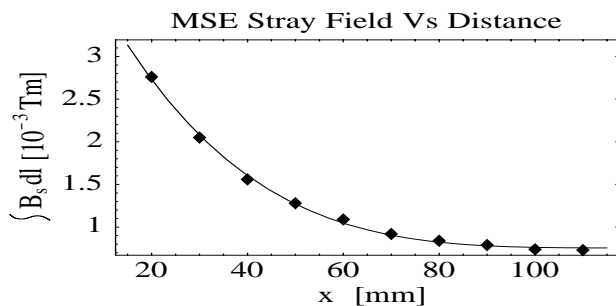
Figure 4. Measured MSE stray field (points) and fit
