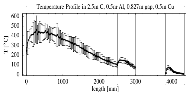
Figure 2. Simulated temperature profile in diluter and MSE coil ( 4.1 \cdot 10^{13} protons, 450 GeV/c, 3.5 \mu m \epsilon_{nh} ).
