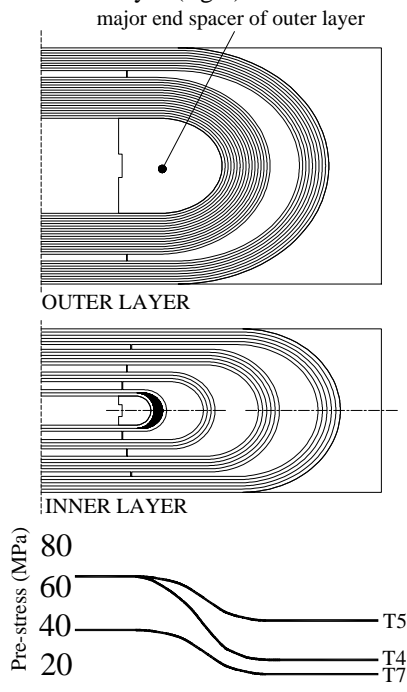
Figure 1: Layout of inner and outer layer ends and azimuthal pressure distribution.
