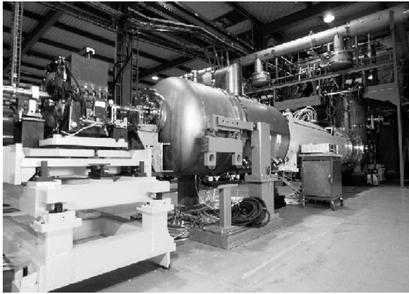
Figure 2: The SSS3 Short Straight Section mounted to cryogenic test station at CERN.
