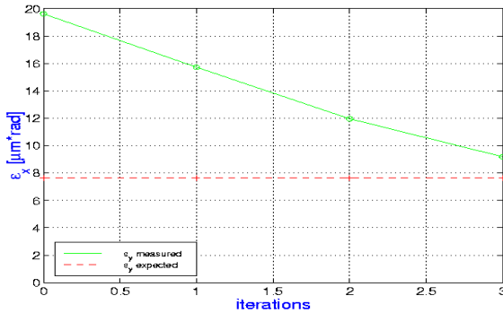
Fig.4: FF vertical emittance as function of Arc-tuning iterations. The expected value comes from the measurement at the end of the Linac plus the contribution from the synchrotron radiation in the Arc
