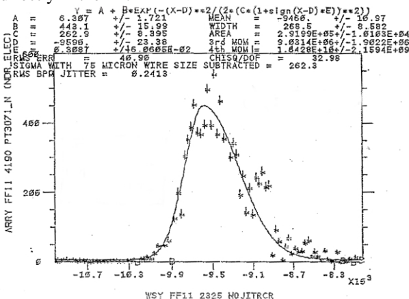
Fig.2a: Typical FF wire scan after optimizing the Linac emittances
