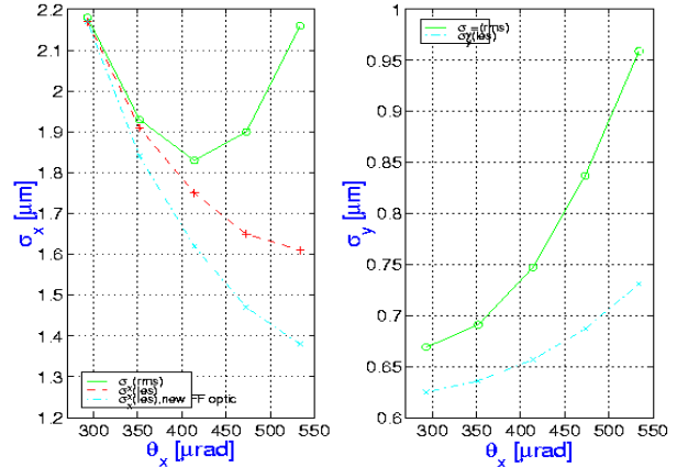
Fig.5: Horizontal and vertical “rms” and “les” spot sizes versus horizontal angular divergence
