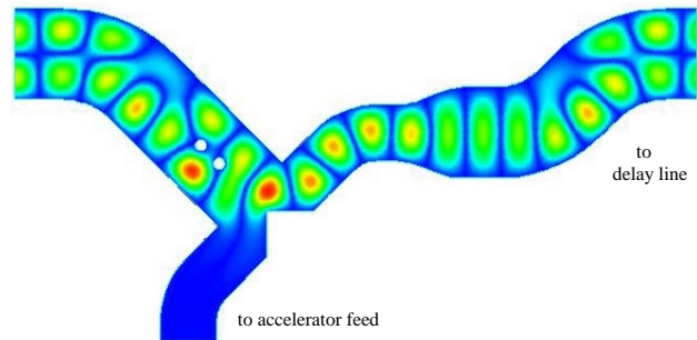
Figure 3: Extractor with jog converter passing TE_{20} . A TE_{10} wave incident from the left would be extracted to the lower port.
