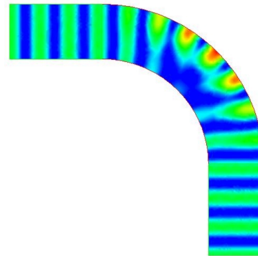
Figure 5: Overheight E-plane bend. No power is left in the coupled TM_{11} mode at the end.
