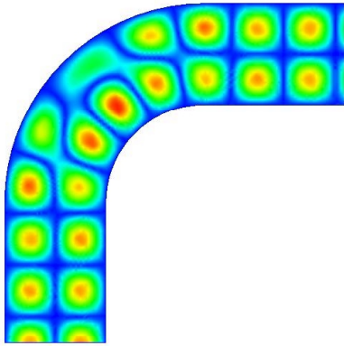
Figure 4: Dual-mode H-plane bend. TE_{10} and TE_{20} pass from input to output unmixed.
