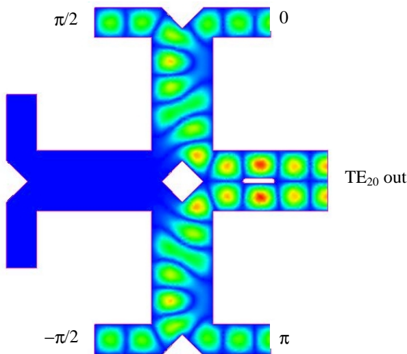
Figure 2: Cross Potent Launcher launching TE_{20} in the right port. Alternate phasings of the inputs send power into TE_{10} or to either of the left ports
