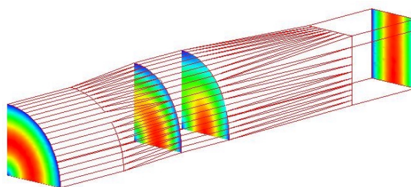
Figure 1: Taper Converter \frac{1}{4} geometry converting circular TE_{01} to rectangular TE_{20} . An incident circular TE_{11} wave would be converted to rectangular TE_{10} .
