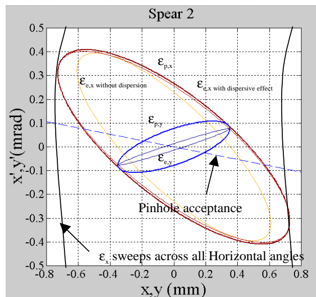
Figure 1: Horizontal and Vertical Emittances in Phase space (vertical for 1% coupling). The 3 horizontal ellipses correspond to electron emittance \epsilon_e , electron emittance including dispersive term \epsilon_{e,d} , \epsilon_p photon beam emittance. The 2 vertical emittances are electron emittance \epsilon_e and the photon beam emittance \epsilon_p .
