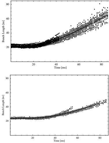
Figure 2: Bunch length during debunching, \gamma = 21.3 (top) and \gamma = 27.7 (bottom). Intensities (2.8 - 4.3) \times 10^{10} .
