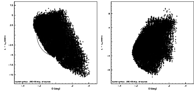
Figure 4: Phase space distribution (ESME) below (left) and above (right) transition 50 ms after injection. |\eta| = 5.2 \times 10^{-4} . Resonant impedance at: f_{res} = 1.6 GHz, Q = 100 , R/Q = 30\ \text{k}\Omega . Bunch: N = 3 \times 10^{10} , \epsilon = 0.24 eVs. Partially hidden curve shows initial bunch.
