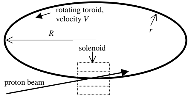
Figure 1: Schematic diagram of the rotating toroid.
