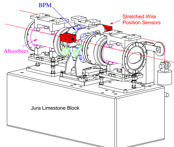
Figure 2: One of the BPM stations with its wire system.
