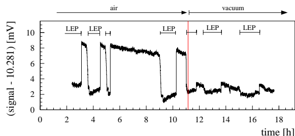
Figure 7: The signal from the sensor (inversely proportional to the distance), after offset subtraction, against time.
