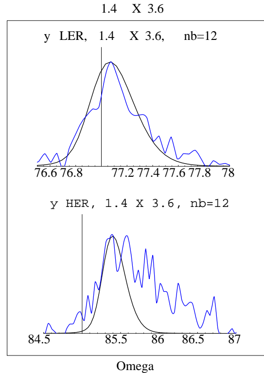
Figure 4: y-spectra of both beams. \sigma_{x,LER} = \sigma_{x,HER} , \sigma_{y,HER} = 4\mu\text{m} , \sigma_{y,LER} = 6\mu\text{m} . No fitting is used in the position of the maximum. HER spectrum is much wider than expected from beam-beam tune spread.
