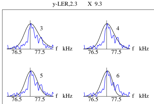
Figure 3: Calculated LER spectra in y-plane for \sigma_{y,HER} = 3, 4, 5, and 6\mu\text{m} at IP. \Sigma_{x,y} are known from luminosity measurements, \Sigma_x = 228\mu\text{m} , \Sigma_y = 7.2\mu\text{m} . \sigma_x are taken equal for both beams. The beam currents 2.3 \times 9.3 mA.
