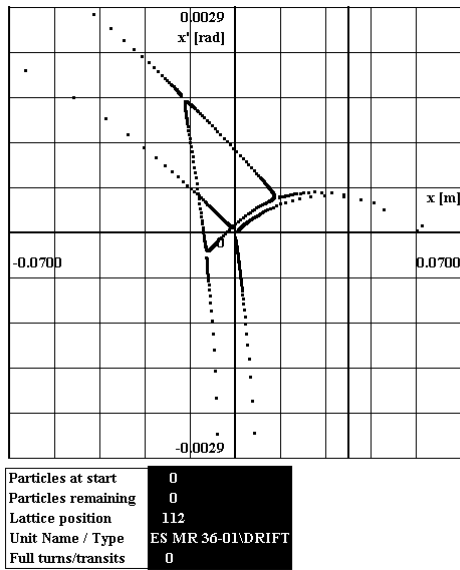
Figure 1: Final screen display from routine for optimisation slow extraction
