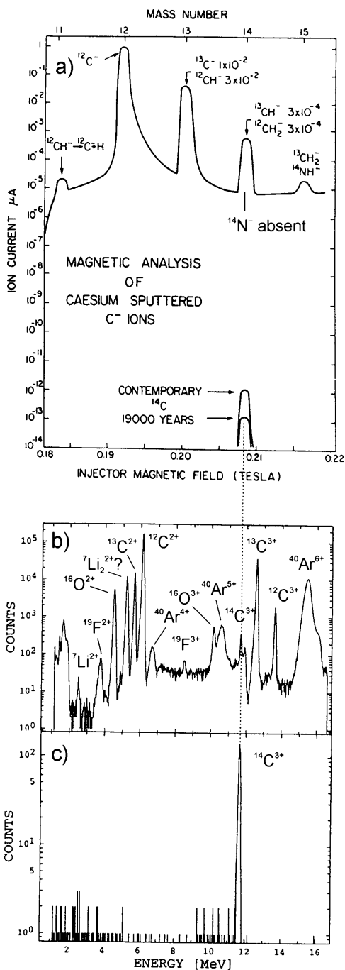
Figure 2: The three steps in the detection of ^{14}\text{C} with AMS at VERA. a) In the negative ion mass spectrum after the ion source the ^{14}\text{C} signal is buried under an enormous background of mass-14 molecules [2]. Most important, however, is the absence of ^{14}\text{N} because nitrogen does not form negative ions. b) After acceleration through the tandem and analysis in the high-energy magnet the energy spectrum measured in the rare isotope detector (Si surface barrier detector) still shows many background peaks. This spectrum is measured with the velocity filter (Wien filter) switched off. c) After final analysis through the Wien filter, a clean ^{14}\text{C} signal emerges.
