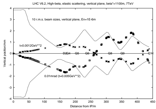
Figure 3: Vertical 10\sigma beam profile and on momentum trajectories starting from the IP with : a) a value of t of 0.0012 \text{GeV}^2 (upper curve), b) a value of t of 0.005 \text{GeV}^2 (lower curve), vs. the distance to the IP for the commissioning emittance and \beta^*=1100 m.
