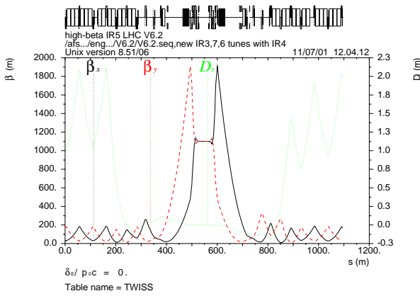
Figure 1: High- \beta optics with \beta^*=1100 m in Ring 1 around IP5 , Version 6.2.
