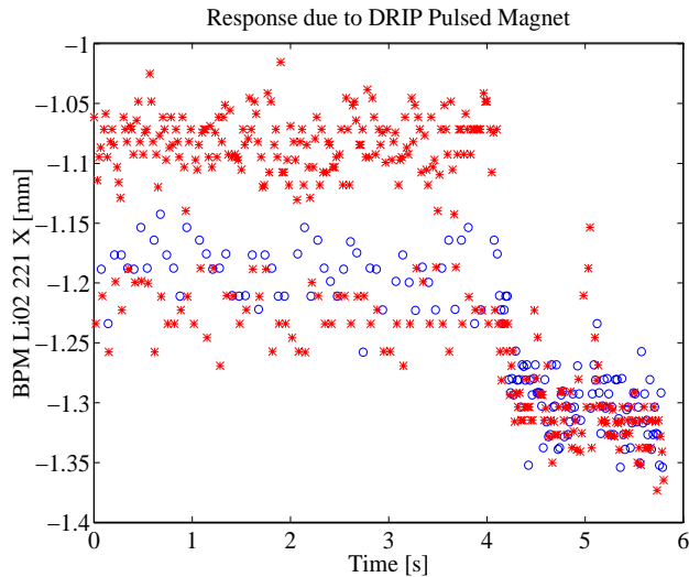
Figure 3: Pulsed magnets don't fully recover at 120 Hz. The transition from "75Hz" (60+15) to 116 Hz occurs at 4 sec. The 200 \mu\text{m} difference could not be fixed yet, but is reduced to only 30 \mu\text{m} at the end of the linac.
