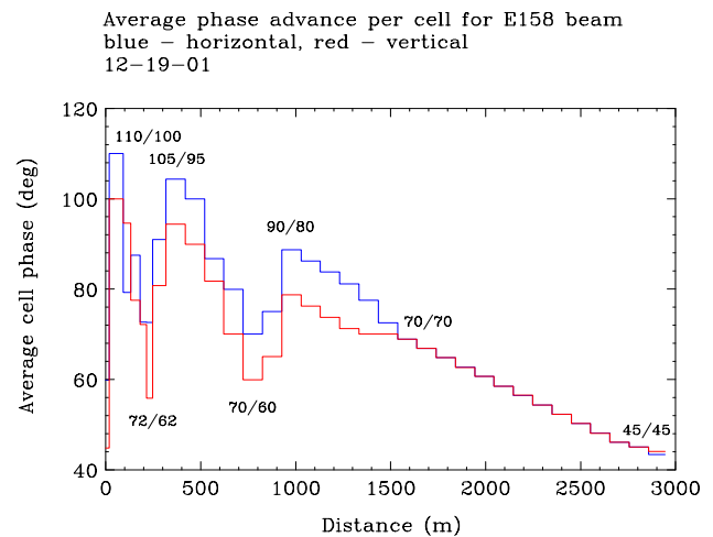
Figure 1: Betatron phase advance per cell in the linac.
