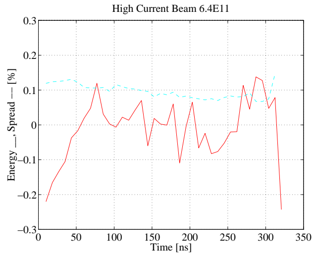
Figure 5: Energy and energy spread along the pulse. The finite rise time of the pulse creates a low energy tail.
