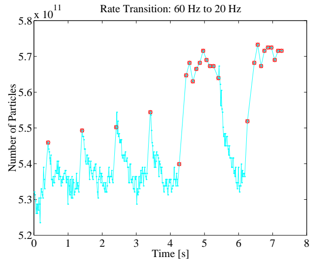
Figure 2: Different rates create different intensities. The rate changed from 60 Hz (58Hz for E-158, 2Hz for PEP-II) to 20 Hz for E-158 at around 4.5 and 6.5 sec. The pulse after PEP and the 20 Hz are marked in red (*). The higher intensities reduce the beam energy.
