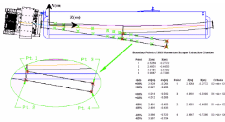
Figure 7: Momentum halo proton extraction
