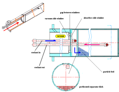
Figure 8: Design layout of the momentum dump
