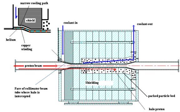
Figure 5: HEBT absorber configuration
