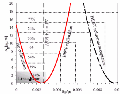
Figure 2: Collimator acceptance
