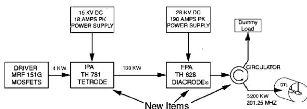
Fig. 1: Major Components of RF Module for Tanks 2 - 4
