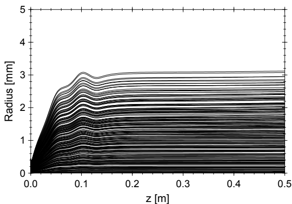
Figure 3: Particle trajectories for a parallel beam in the complete set-up. 200 sample particles are used in the simulation.
