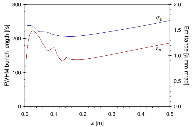
Figure 4: Bunch length and emittance evolution for a parallel beam.
