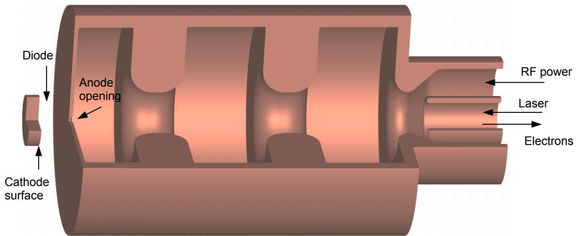
Figure 1: 3D schematic of the rf booster. The diode is shown, not to scale, on the left. The rf power enters the cavity between the inner and outer conductor shown at the right. The inner conductor is hollow to allow the electron beam to pass through and is also used to send the laser beam through the anode opening onto the cathode surface of the diode.
