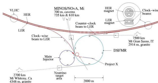
Figure 1: Outline of proposed FNAL accelerator complex
