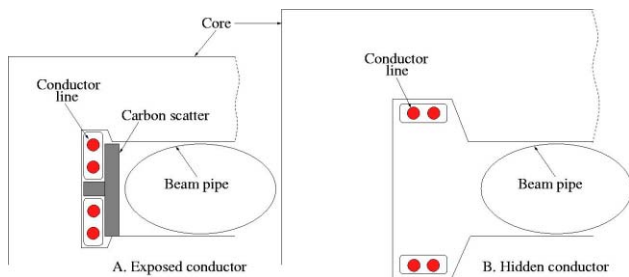
Figure 3: Options for conductor placement within a core
