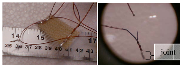
Figure 1: To the determination of shortest allowed length of SC wire joint.
