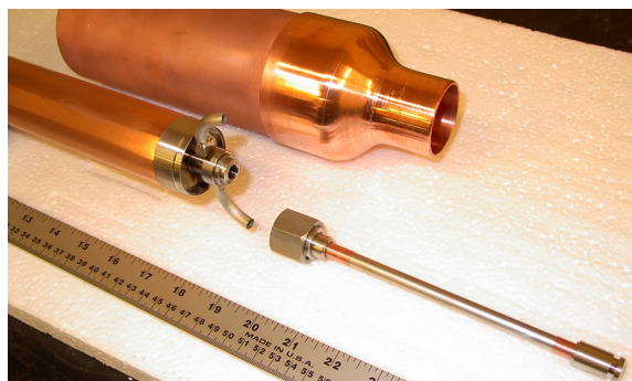
Figure 5: Cold mass, transition to the room temperature flange, part of 70 °K shield.
