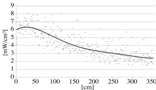
Figure 8: Peak of energy deposition in the first cable of Q0B with liner.
