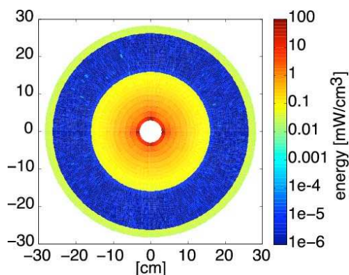
Figure 6: Energy deposition in Q0A with liner.
