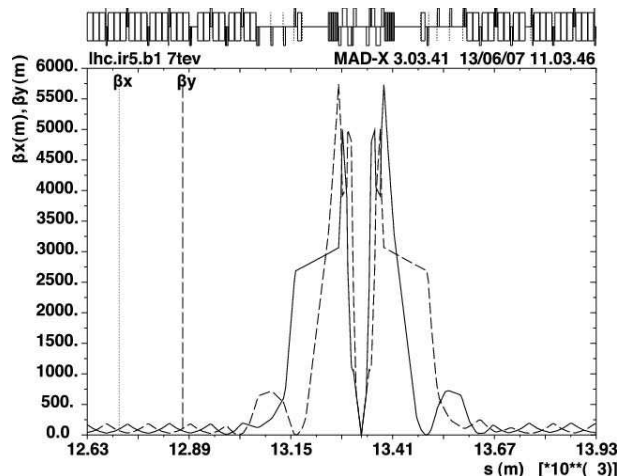
Figure 2: \beta function with Q0 and with \beta^* = 0.25 m.
