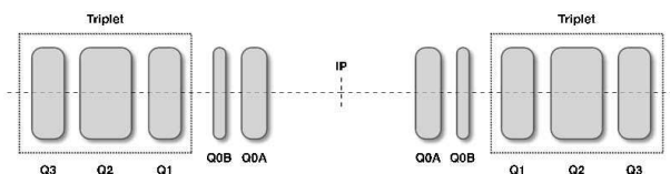
Figure 1: Q0 Layout.
