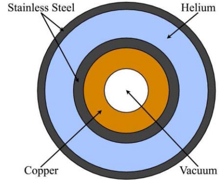
Figure 3: Magnet schematization for FLUKA.
